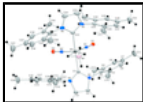
Fig. 1. View of the title compound showing the labeling of the non-H atoms and 30% probability ellipsoids.
